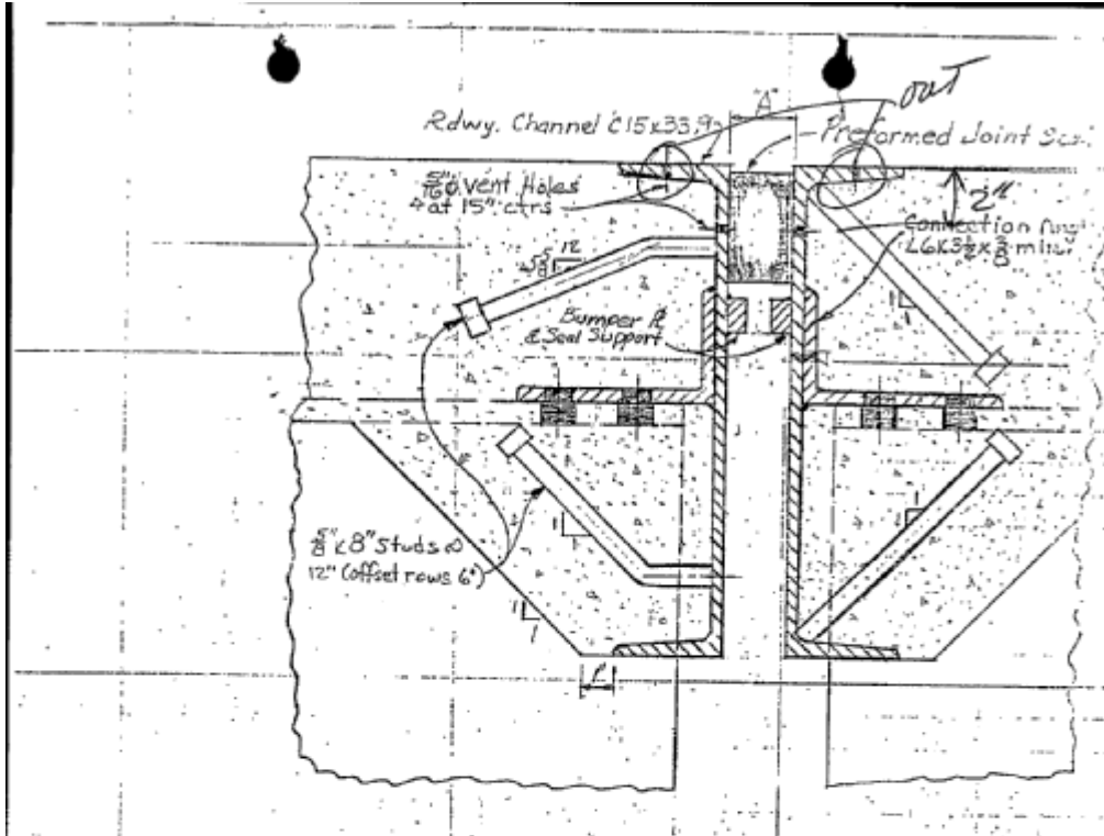
JOINT AT INTERMEDIATE BENT. Scale: 3"=1'-0"
