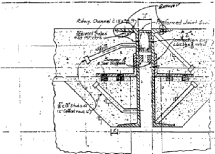
JOINT AT INTERMEDIATE BENT Scale: 3" = 1'-0"
