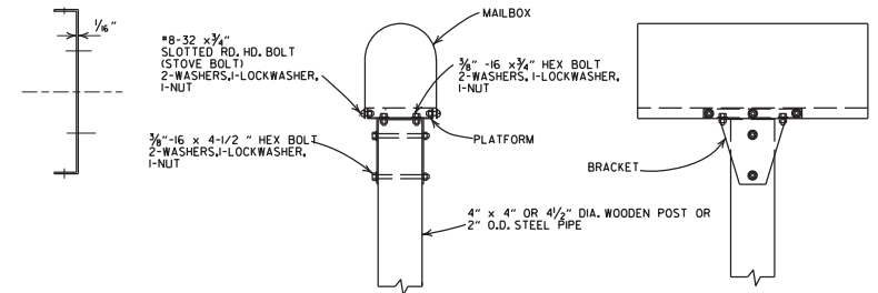
SINGLE INSTALLATION
