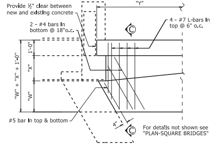
DETAIL X 3/8" = 1'-0"
