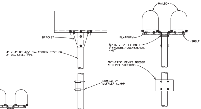
DOUBLE INSTALLATION
