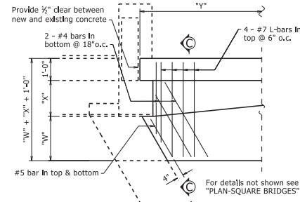
DETAIL X
