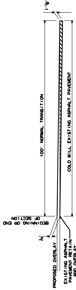
DETAIL FOR TRANSITIONS
