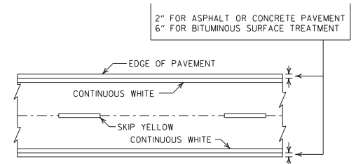
PAVEMENT EDGE LINE MARKING
