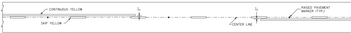
SOLID LINE STRIPING ON ASPHALT PAVEMENT
