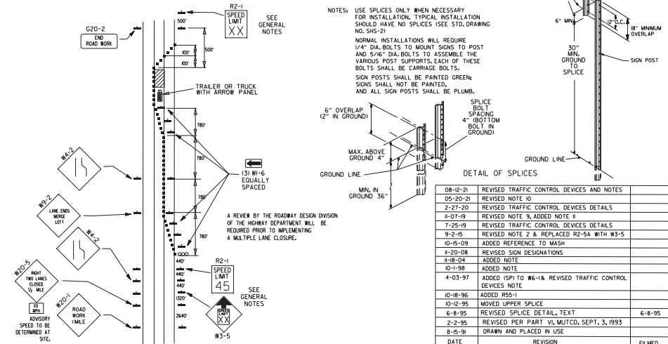
(D) TYPICAL APPLICATION - CLOSING MULTIPLE LANES OF A MULTILANE HIGHWAY.
