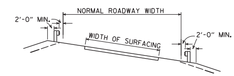
DETAILS SHOWING POSITION OF GUARDRAIL ON HIGHWAY
