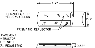
DETAIL OF STANDARD RAISED PAVEMENT MARKERS
